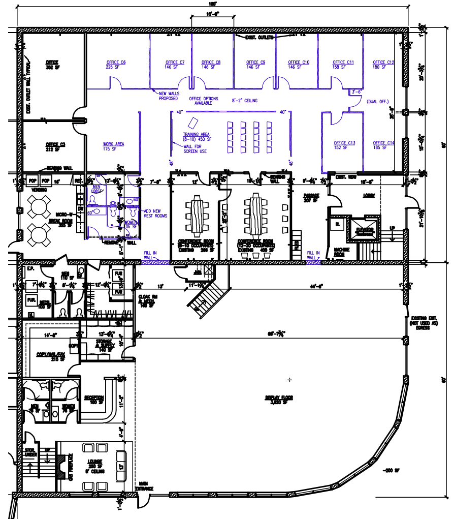
FIRST FLOOR PLAN 1/8" 6,000 sf 5,800 sf 11,800 sf
