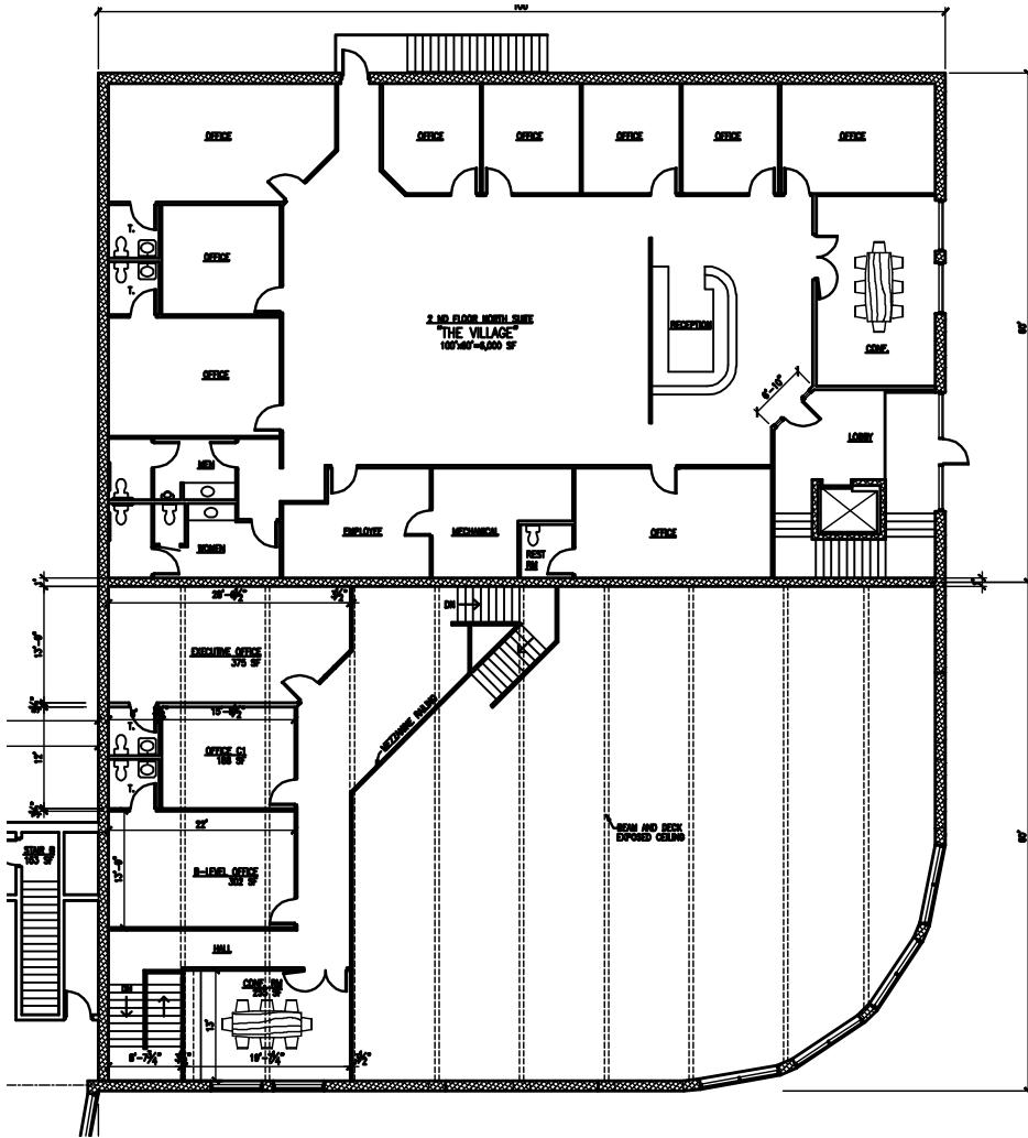
MEZZANINE & SECOND FLOOR PLAN 1/8" 6,000 sf 2,000 sf 8,000 sf
